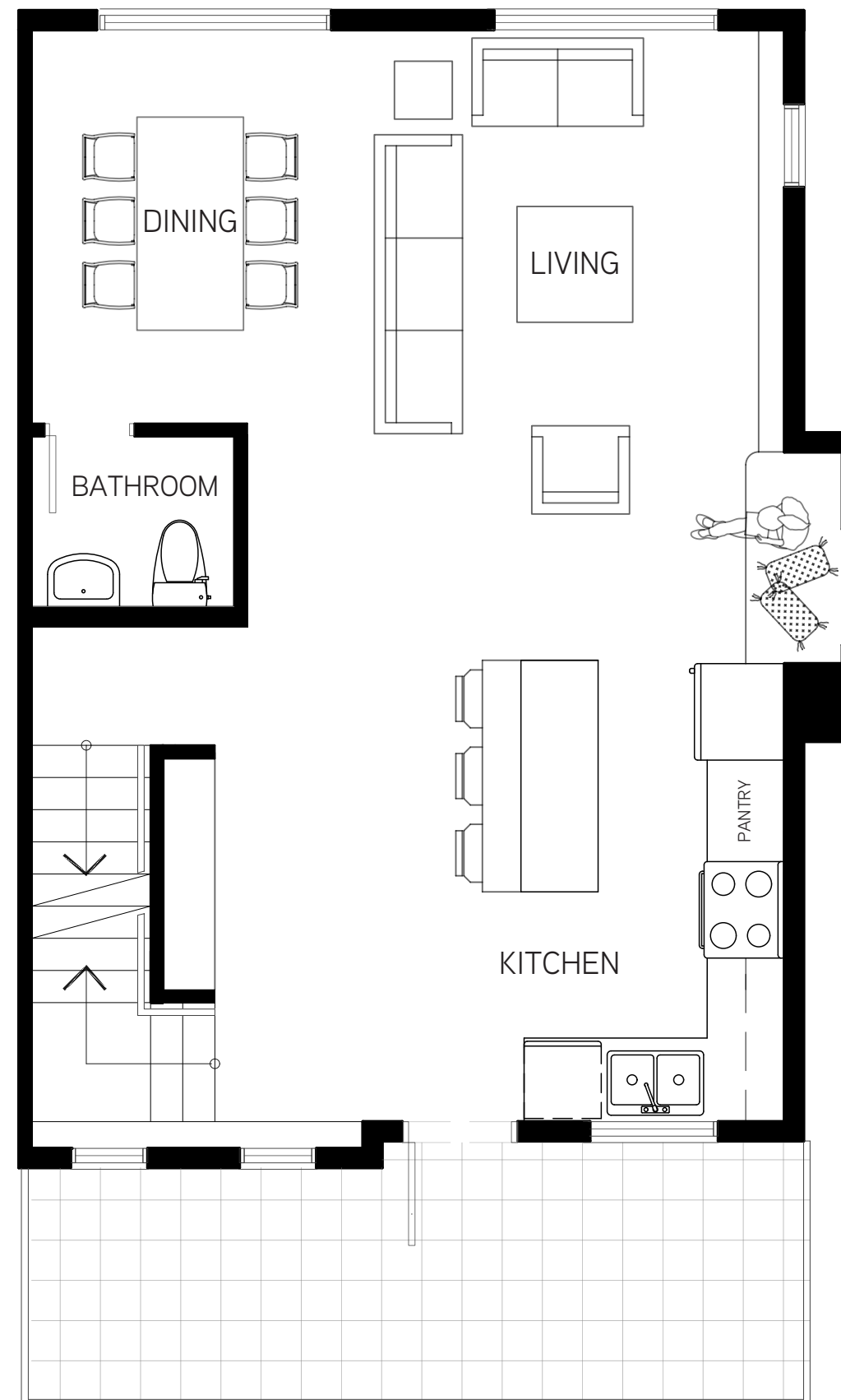
SECOND FLOOR
