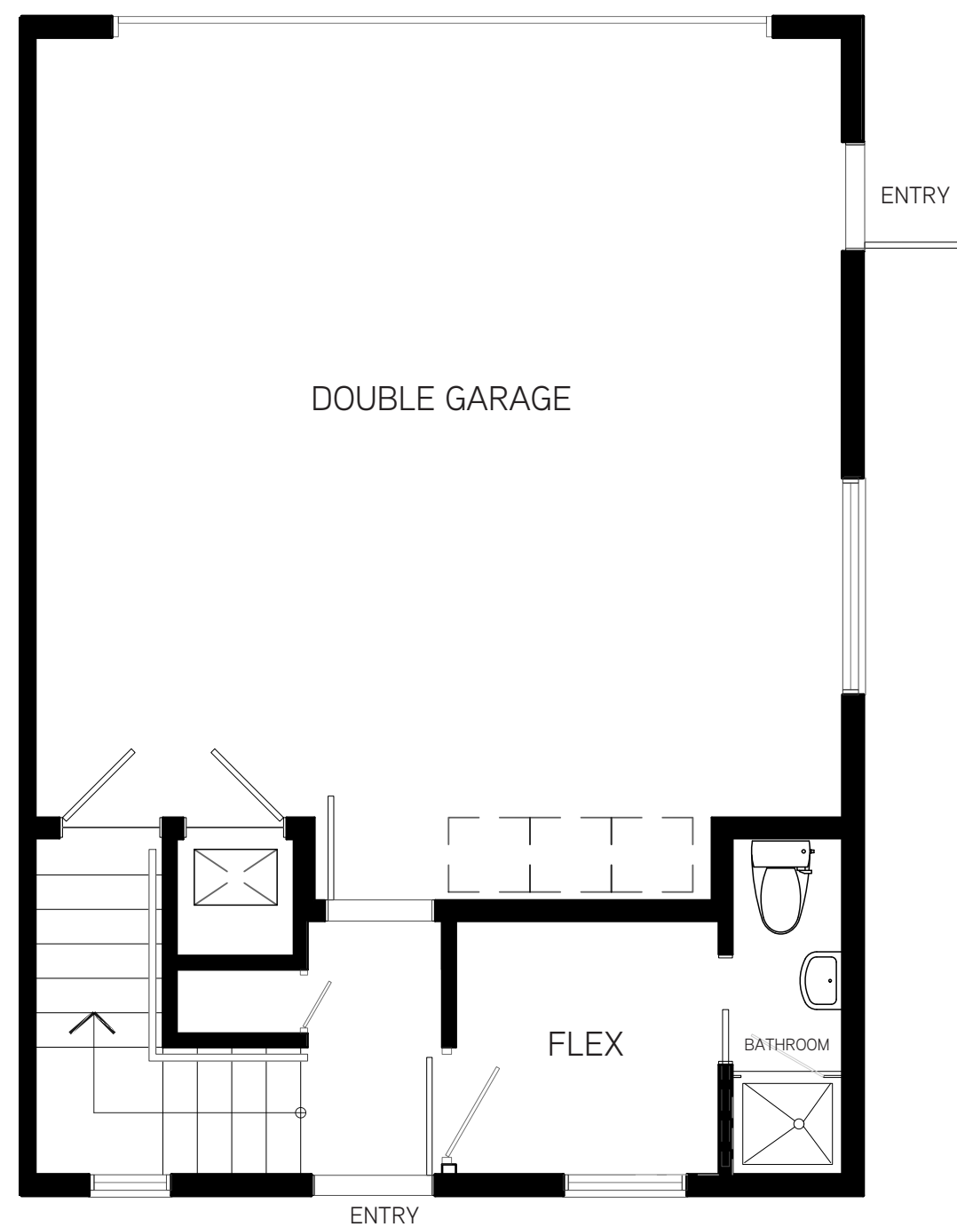
MAIN FLOOR
