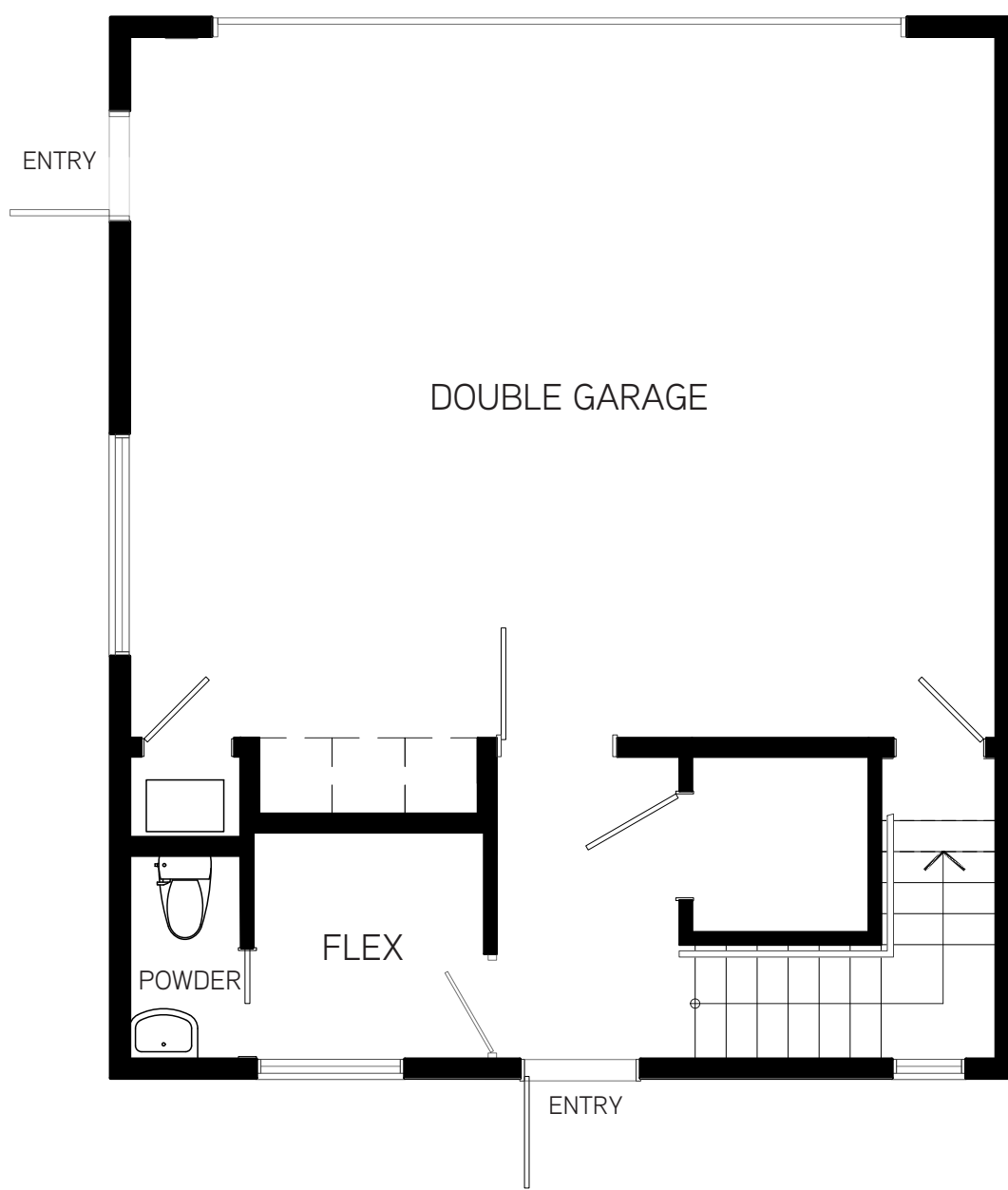
MAIN FLOOR
